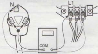
Figure 4. Plug-to-terminal connections.
