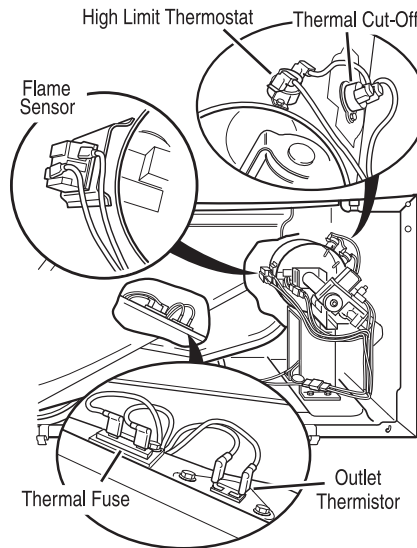
Gas Dryer
