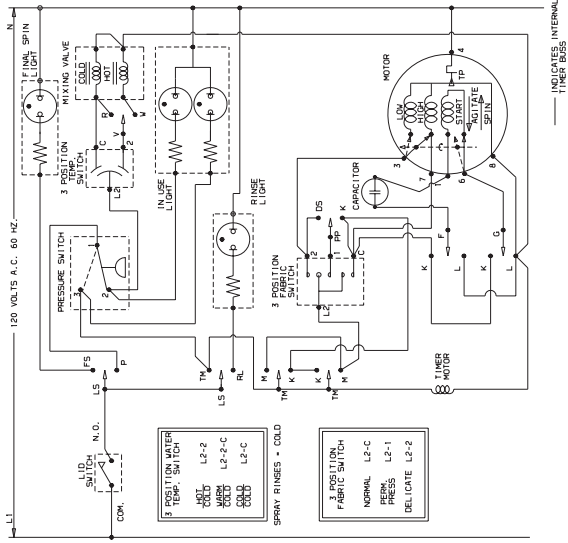
INDICATES INTERNAL WIRING SCHEMATIC
