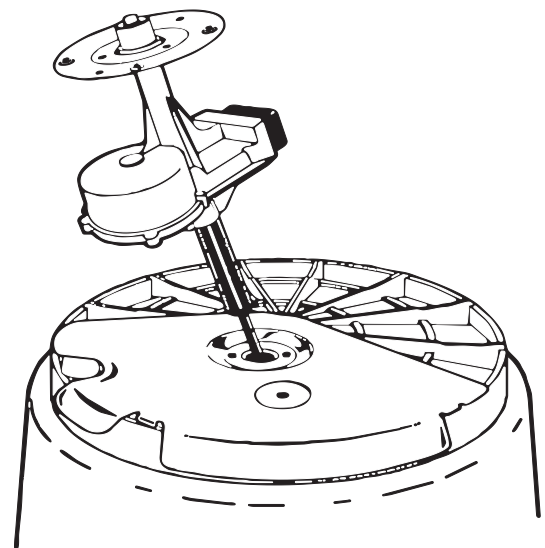
REMOVE TRANSMISSION
