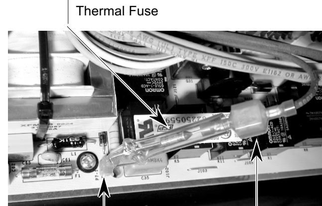
Connector P7-1
