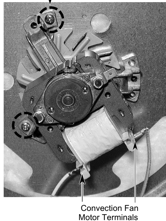
Convection Fan Motor Rear Screw (1 of 2)
